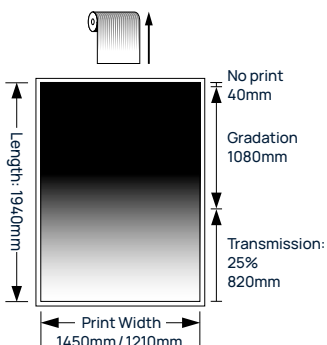
SH2SSIM-S (Single gradation type)
