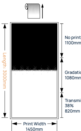
SH2SSIM-S2 NEW (Single gradation type)
